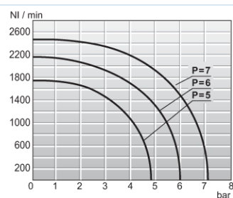
Flow diagram 1/4"
