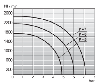
Dijagram protoka 1/4"
