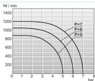
Dijagram protoka 1/8"
